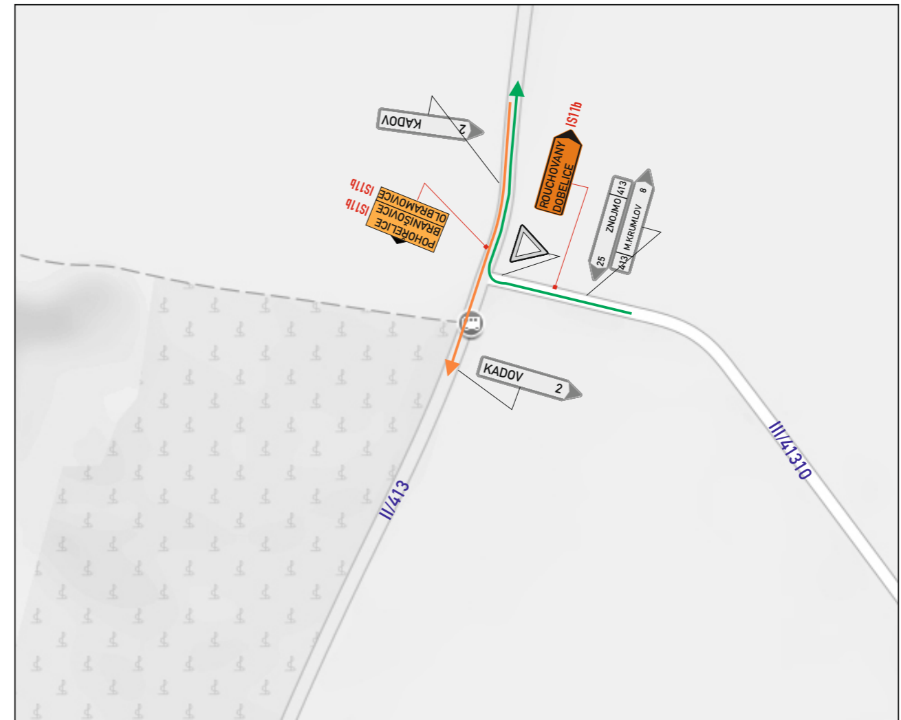
DETAIL 6:
