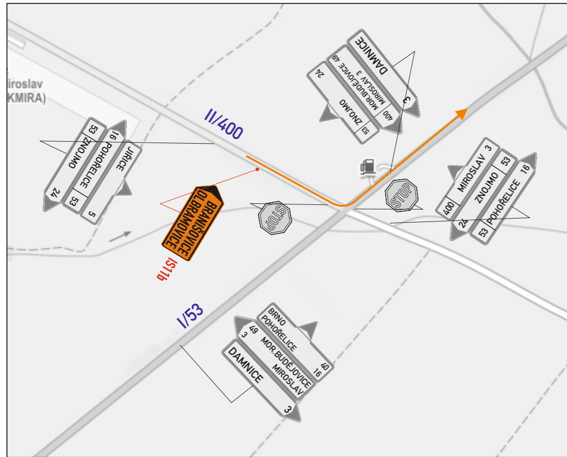
DETAIL 10:
